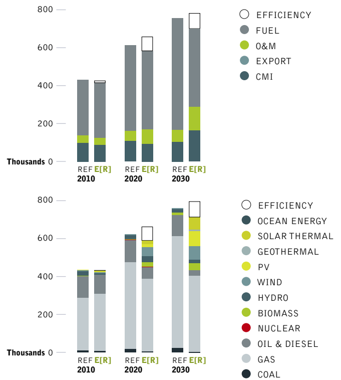
figure 3.26: middle east: jobs by type and by specific technology in 2010, 2020, and 2030
